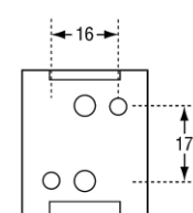
Mounting Bracket
