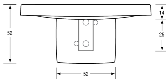
Mounting Bracket
